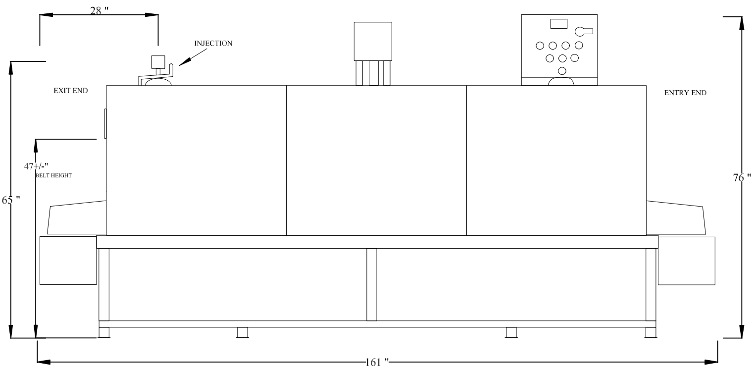
FRONT VIEW
